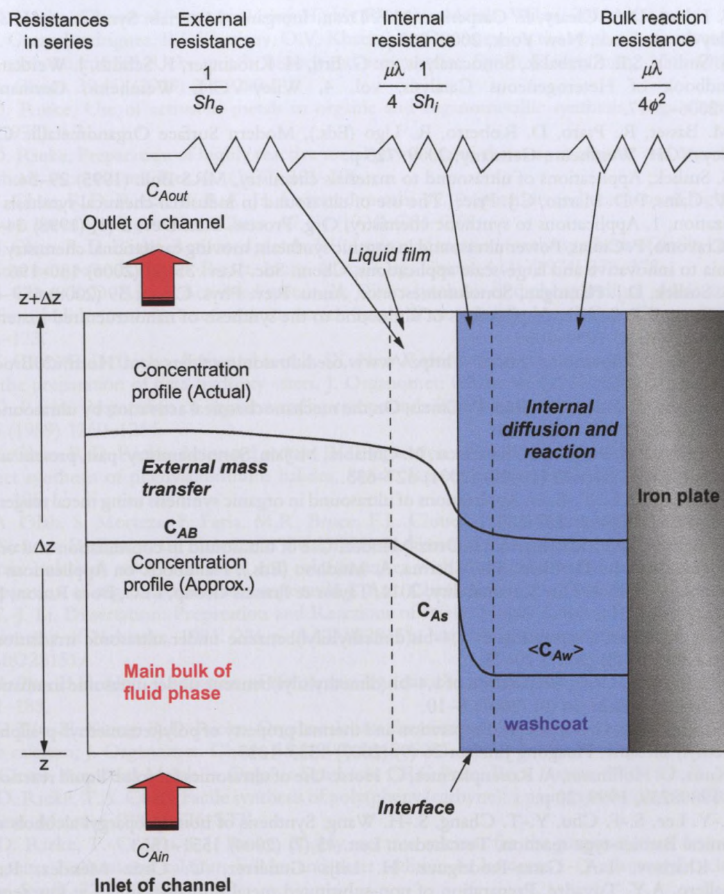
Fig. 11 Schematic diagram of the control volume that illustrates the fluid-solid mass-transfer during a chemical reaction in the washcoat with resistances using a series approach.
